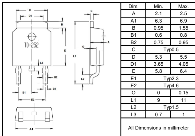
T0-252
