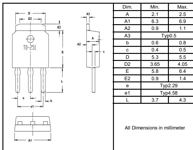
T0-251
