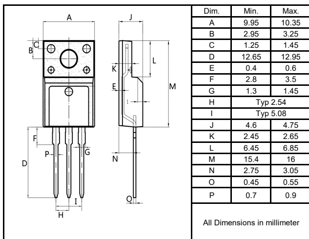
T0-220F
